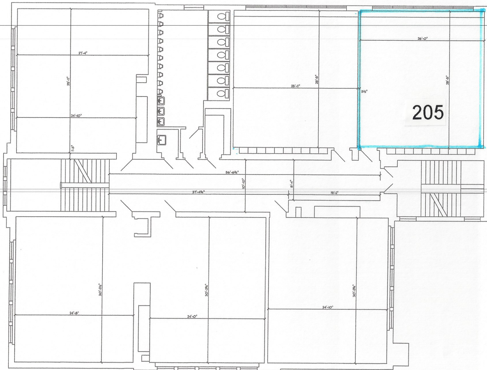
EXISTING 1ST FLOOR PLAN, GOOD SHEPHERD SCHOOL
