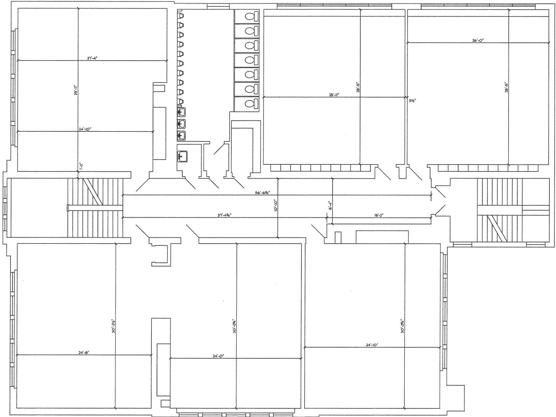
EXISTING 1ST FLOOR PLAN, GOOD SHEPHERD SCHOOL
