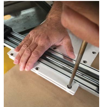
Figure 3 Place over clamp, Loosen all three screws. Squeeze and then tighten.
