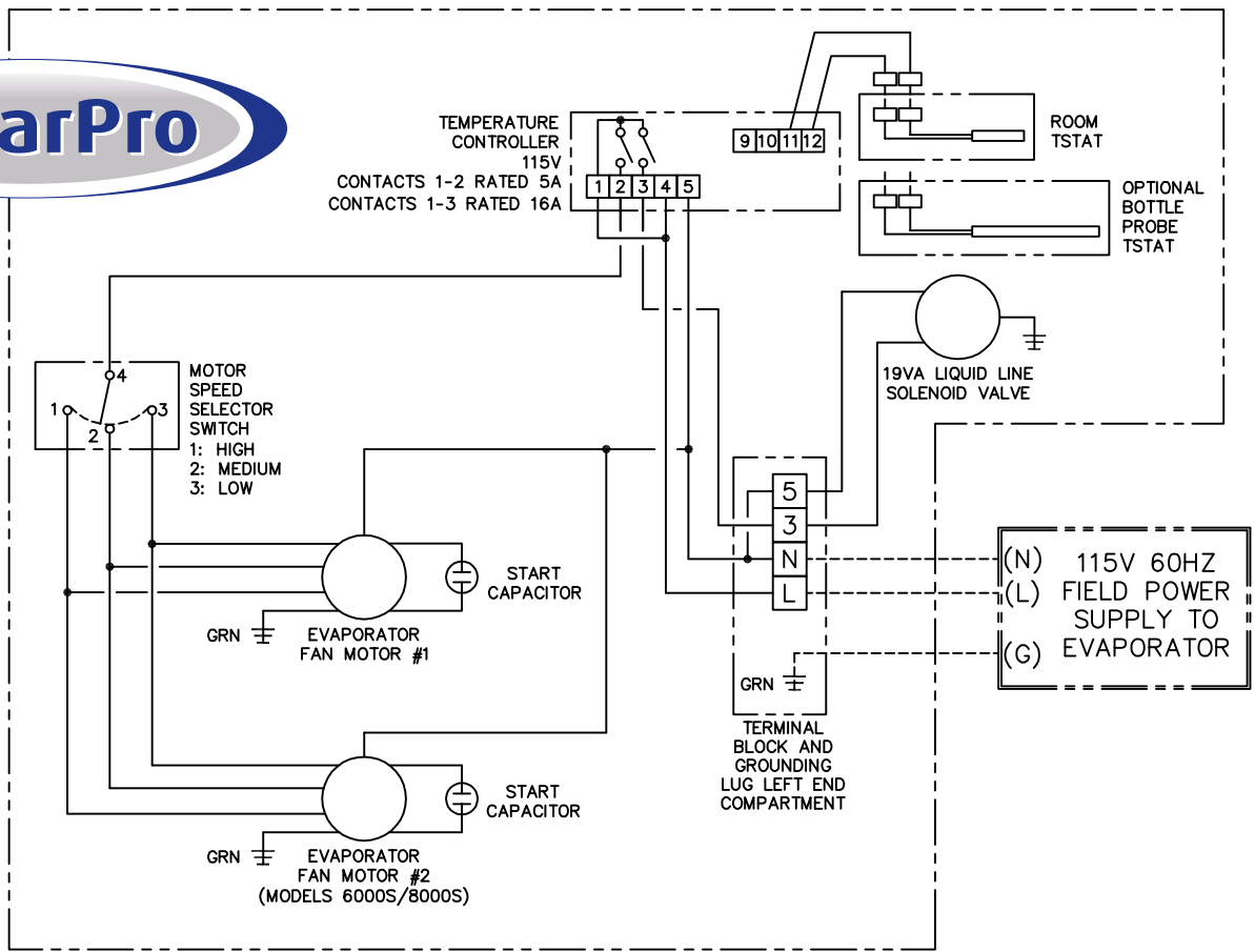
EVAPORATOR UNIT WIRING DIAGRAM
