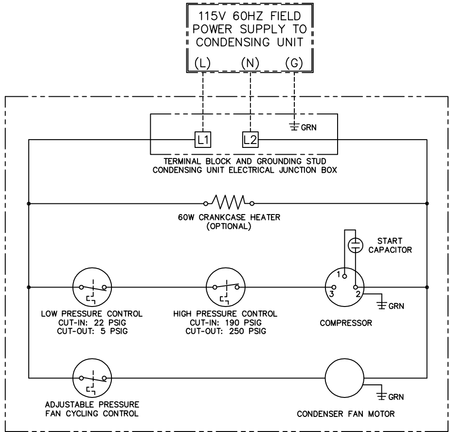
CONDENSING UNIT WIRING DIAGRAM
