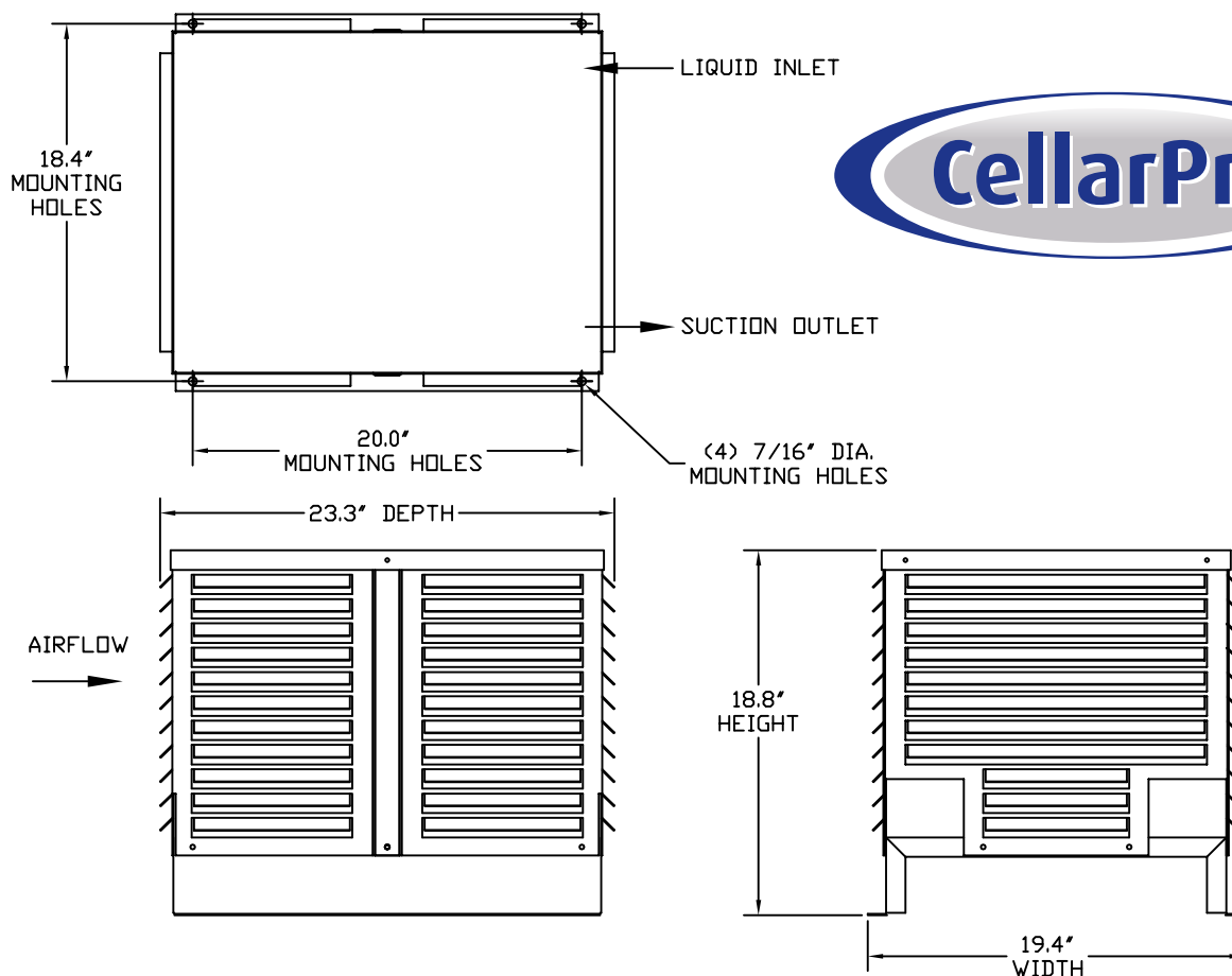
CONDENSING UNIT WITH HOOD (OUTDOOR)
