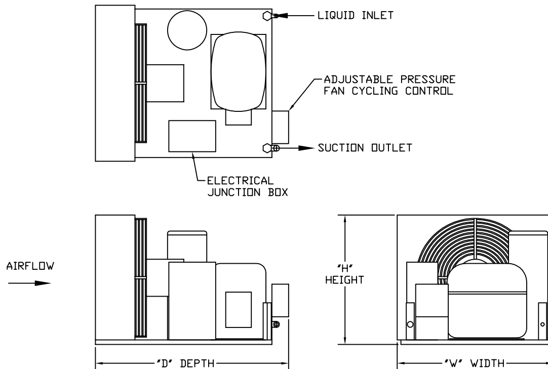
CONDENSING UNIT (INDOOR)
