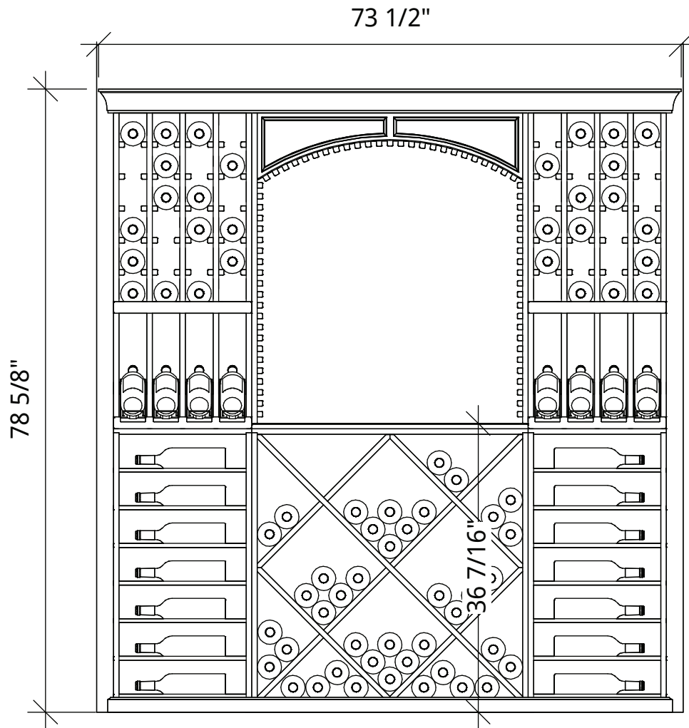
1 Elevation 1 NOT TO SCALE
