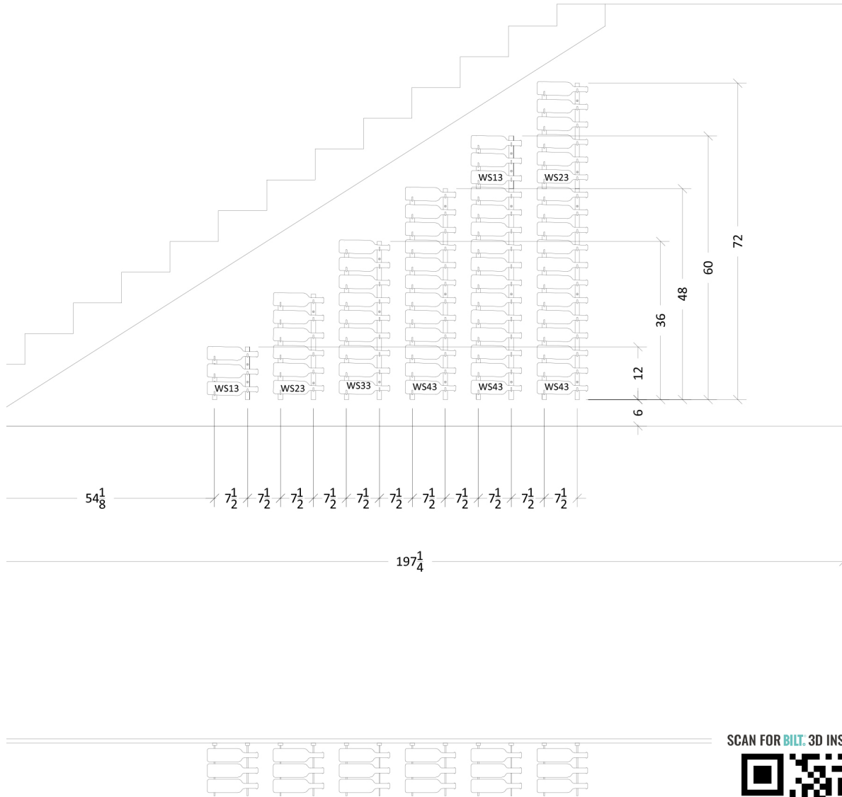
1 PLAN AND ELEVATION Scale: 3/8" = 1'-0"
