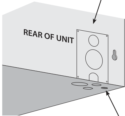
Thermostat wire routing for 24V thermostat (NOT INCLUDED)
