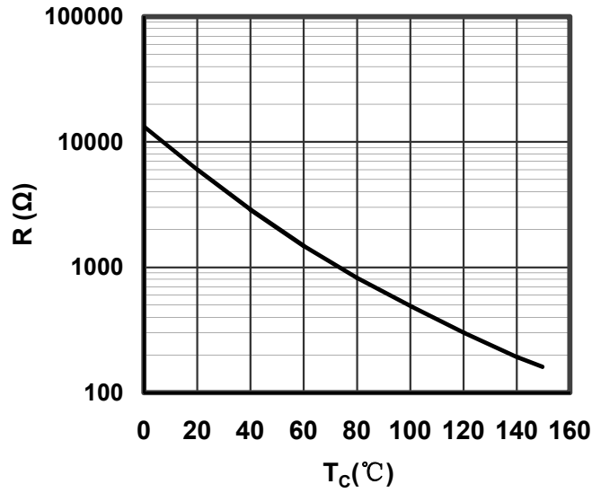
Figure 13. NTC Characteristics
