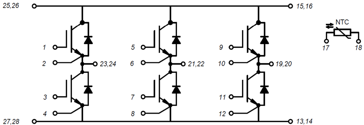
Figure 14. Circuit Diagram
