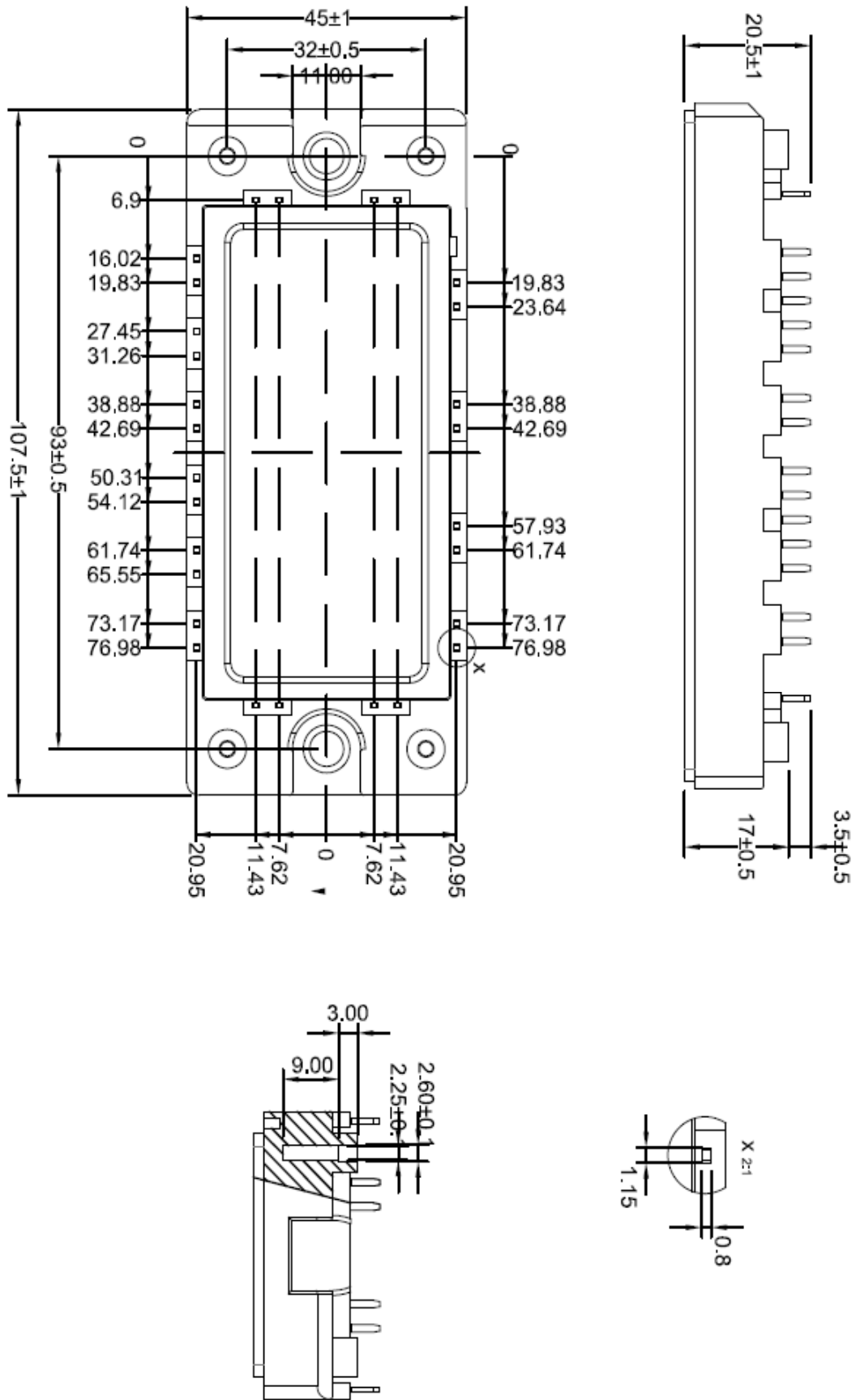
Dimensions in (mm) Figure 15. Package Outline
