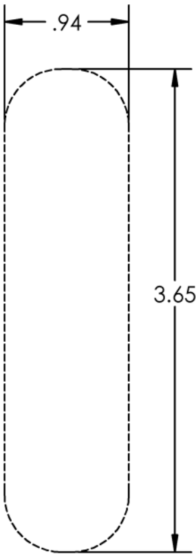
MOUNT FOOTPRINT
