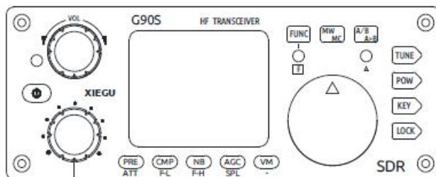
Multi-function adjustment knob
