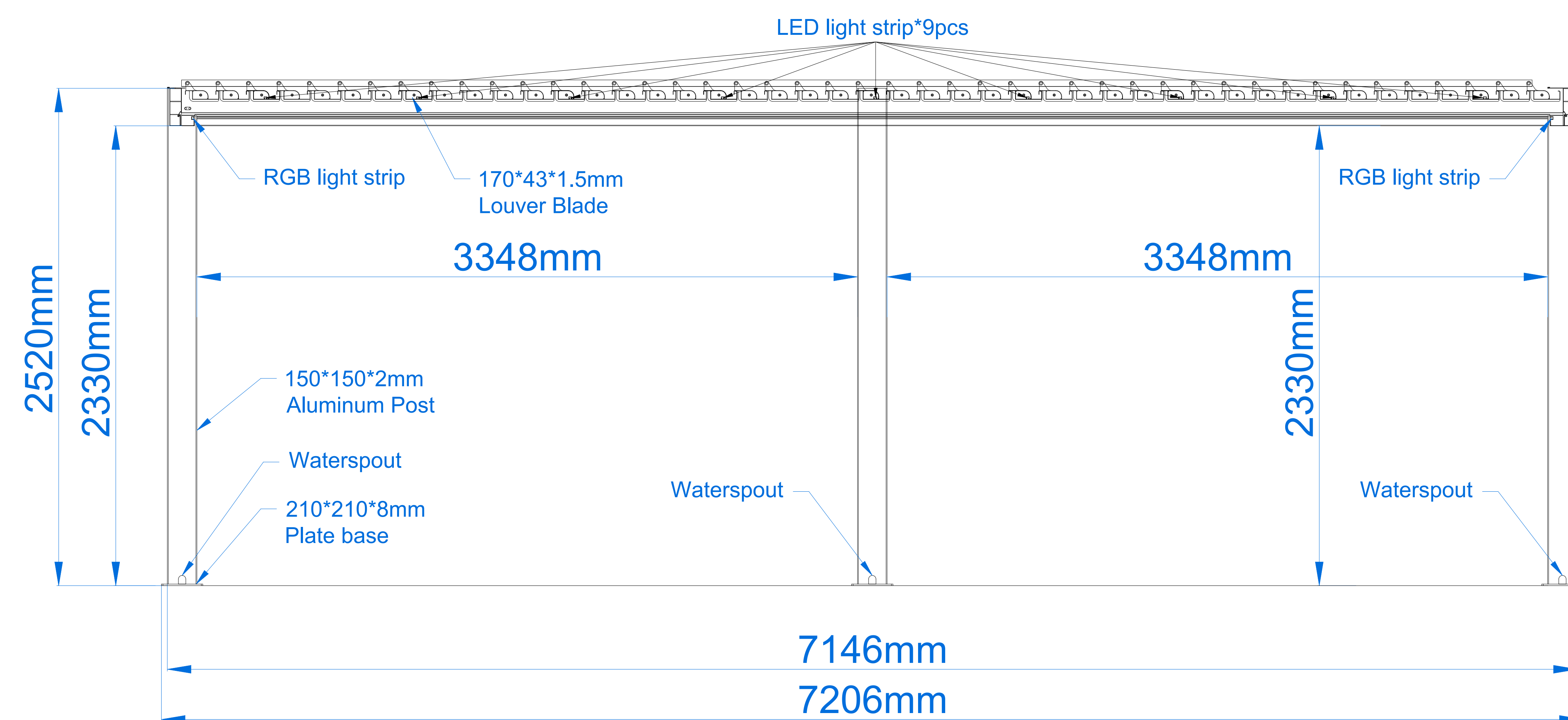
ELEVATION VIEW
