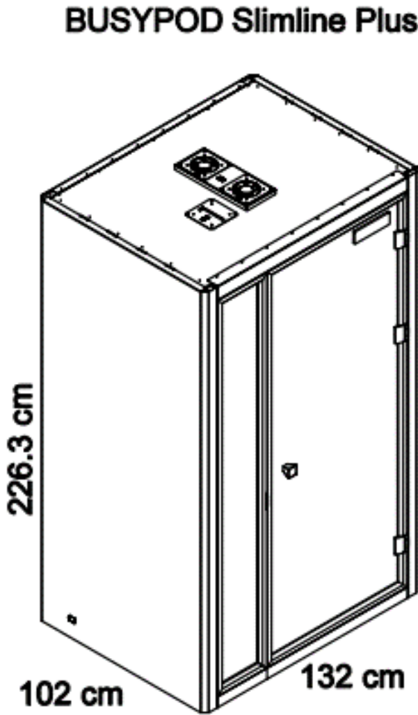
Figure 3.1 Technical Drawing of BUSYPOD Slimline Plus
