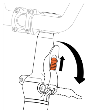
Releasing the latch on the stem riser
