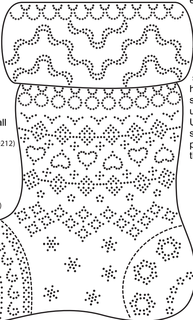
Picot V small stars
