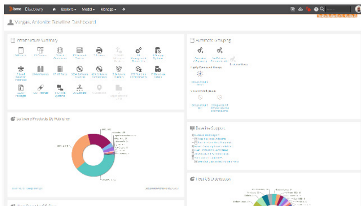
Baseline dashboard provides insightful overview and drill-down access into discovered software and hardware components.
