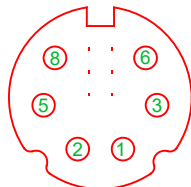
WIRE ENTRY KMDLAX -6P
