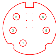
PIN VIEW KMDLAX-5P
