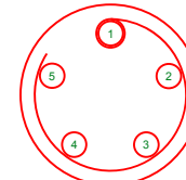
5 WAY SC PIN VIEW
