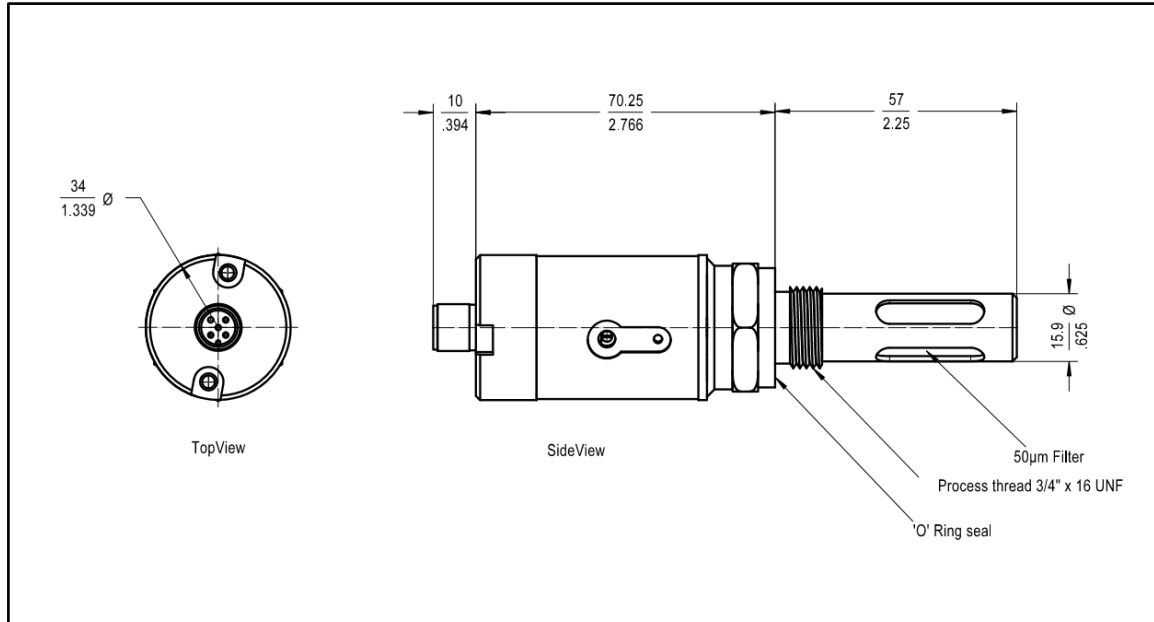
Edgetech Instruments' AcuDew Moisture Transmitter
