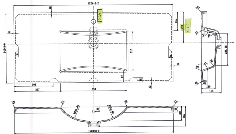
SINK DETAIL
