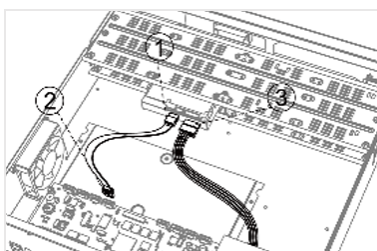
Figure 1-3 Connect Cable
