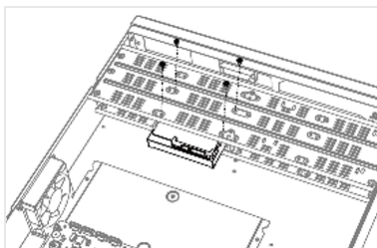
Figure 1-2 Fix HDD
