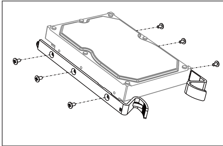
Figure 1-4 Fix Mounting Ears to HDD
