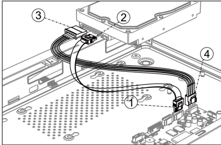
Figure 1-8 Connect Cables
