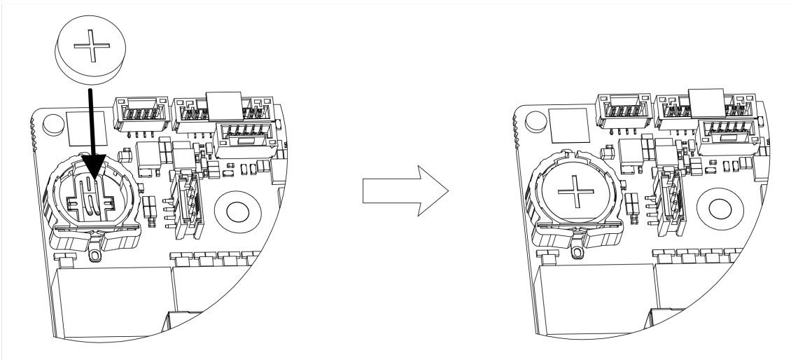
Figure 1-11 Replace Battery
