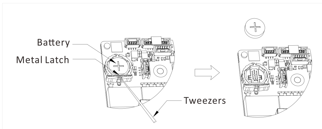
Figure 1-10 Remove Battery
