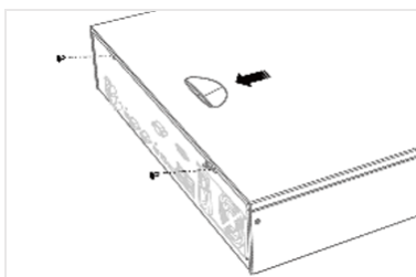
Figure 1-1 Remove Cover
