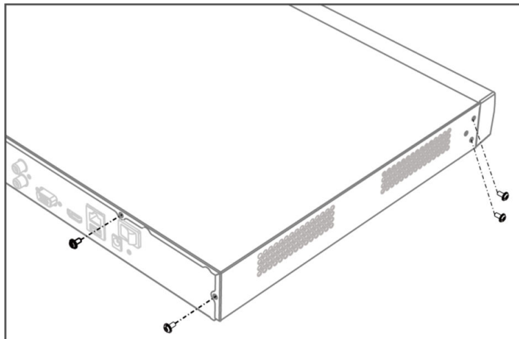
Figure 1-7 Remove Cover
