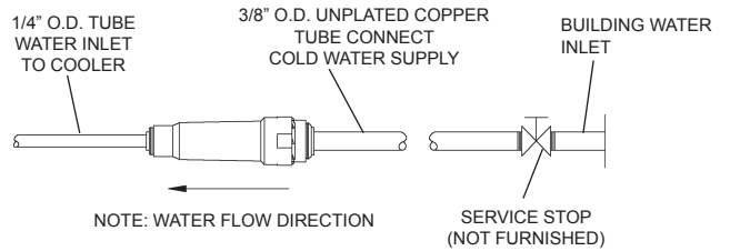
Figure 3– Water Supply Connections
