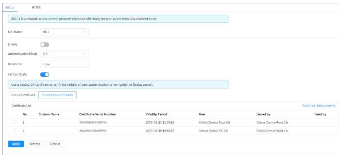
Figure 9-4 802.1x (TLS)
