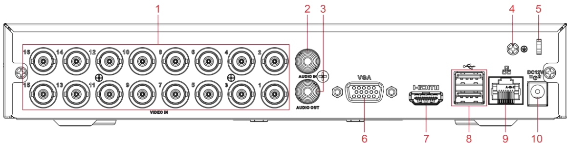
Figure 3-21 Rear panel
