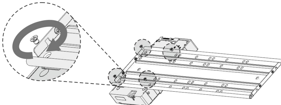
Figure 2-19 Fix HDD
