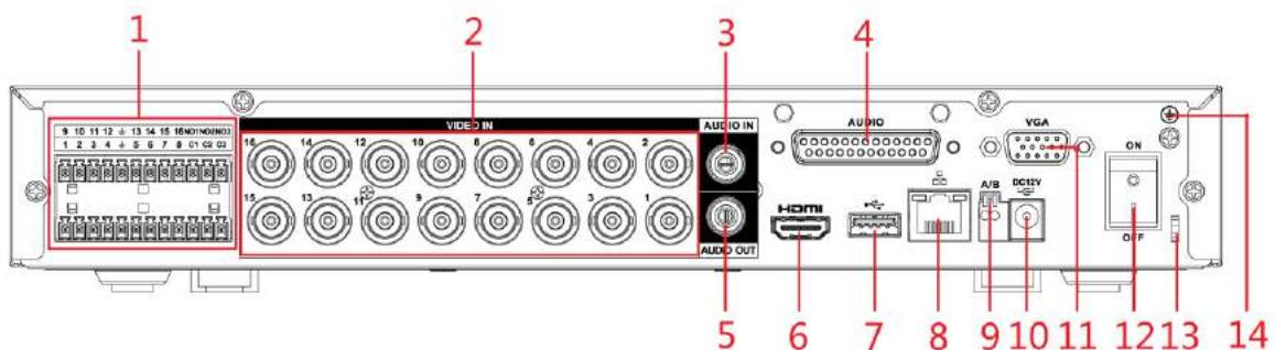
Figure 3-12 Rear panel
