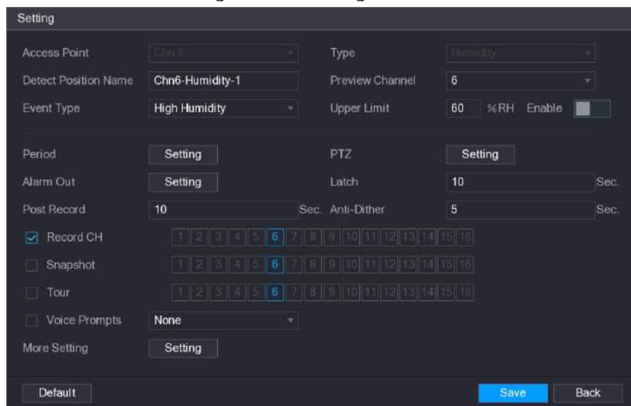
Figure 5-206 Setting
