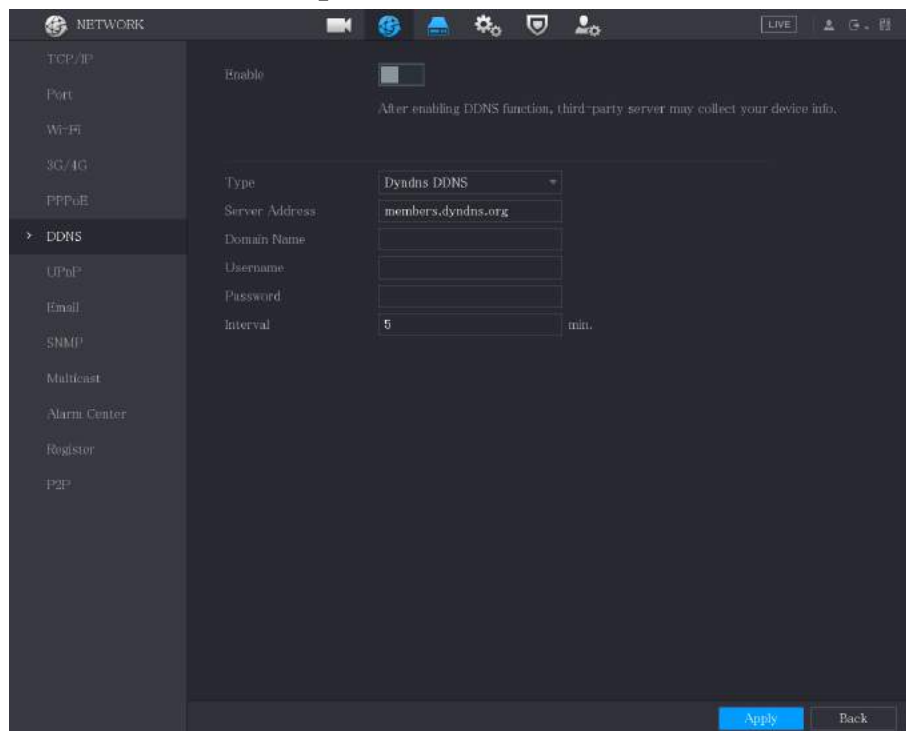
Figure 5-224 DDNS
