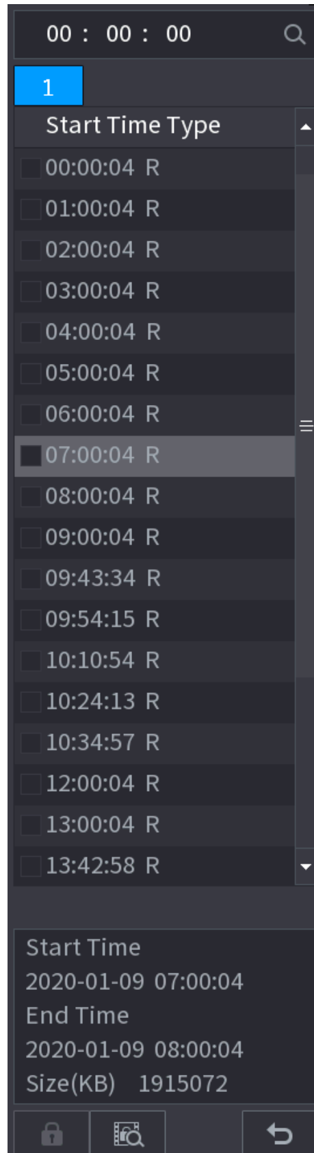
Figure 5-109 File list
