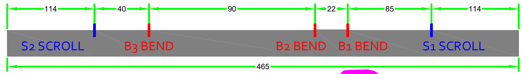
FIG 1 FLAT STRIP NOT TO SIZE
