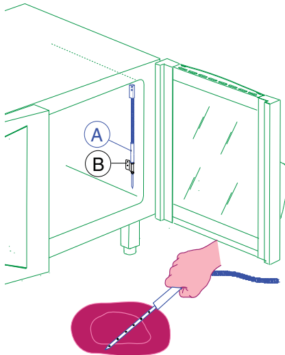
—————MULTIPOINT 6-sensor core probe
