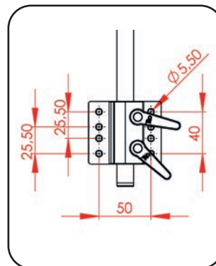
Mounting Plate Measurements In mm
