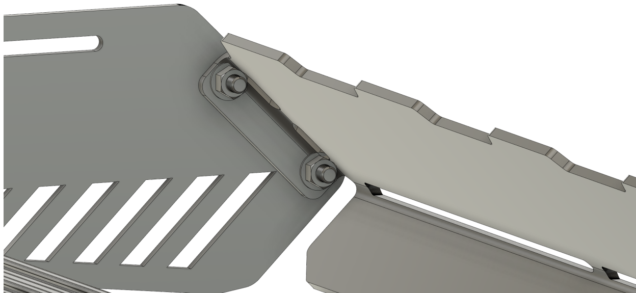
Figure 13 Fairing installation Driver Side 2001 Shown
