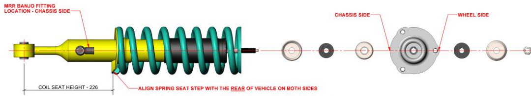
TOYOTA HILUX (2005-ON) RIGHT HAND STRUT SHOWN
