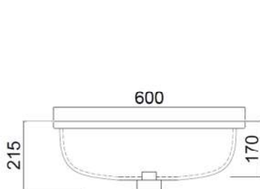
AURORA 600 × 400 × 170 MM
