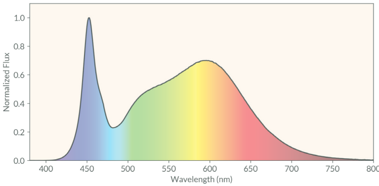
Spectral Power Distribution –UX
