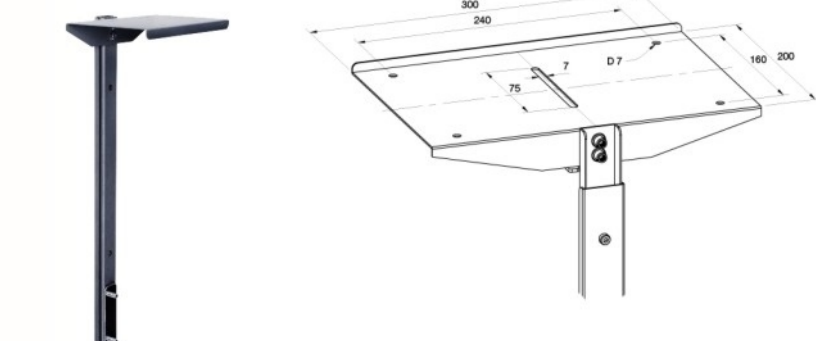
Camera Holder
