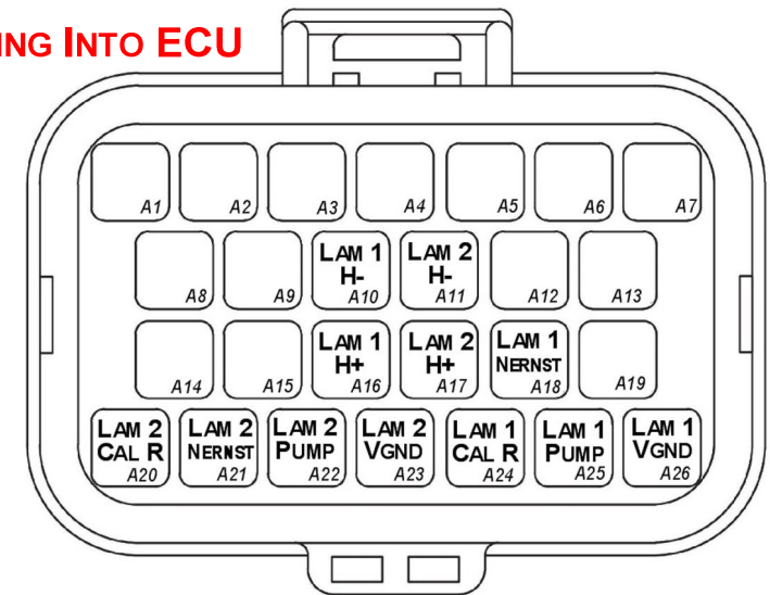
CONNECTOR A
