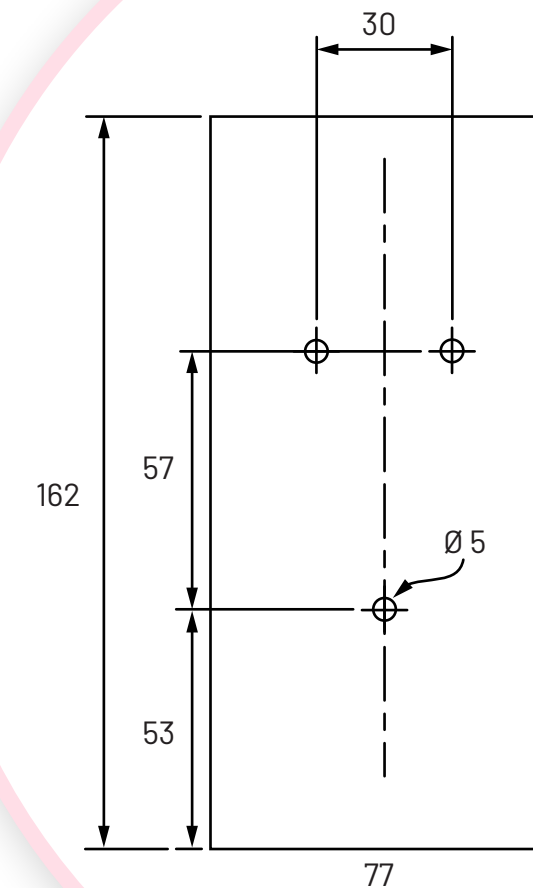
Rear view (showing fixing points)
