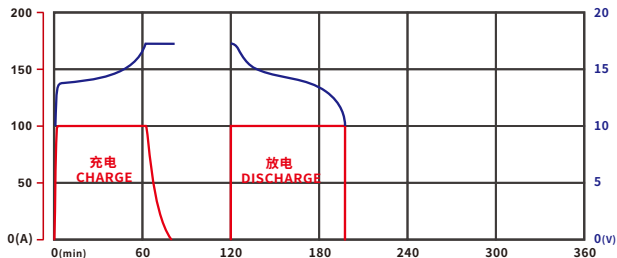
TSWB-LP12V100AH CHARGE AND DISCHARGE BY 100A AT TEMPERATURE OF 25°C
