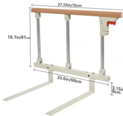
BED SIDE RAILING SUPPORT
