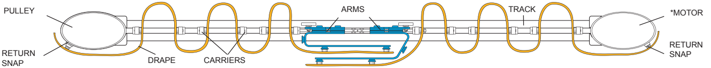
Bottom-up view of track and drape assembly
