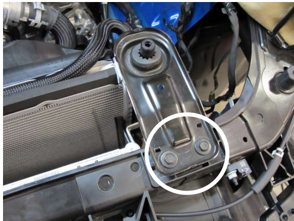
Fig. 3-a: Remove Upper Radiator Brackets
