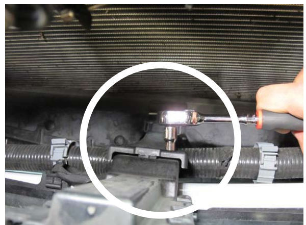
Fig. 1-r: Remove 2x 5.5mm-Headed Fasteners
