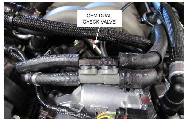
Fig. 8-k: 3/8" Hose Attachment
