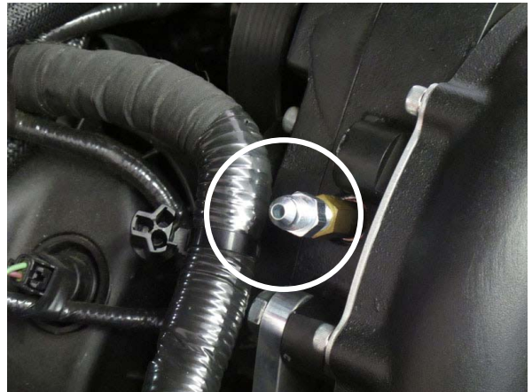
Fig. 11-b: -4AN Oil Feed Fitting Installed
