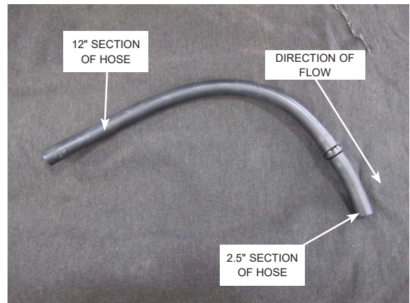
Fig. 8-h: Hose Arrangement w/Provided Check Valve
