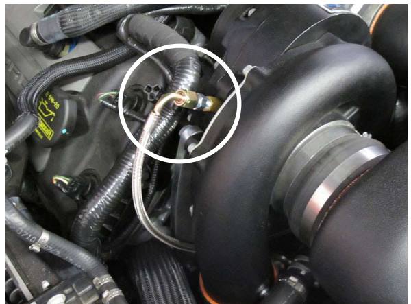
Fig. 11-c: 90° Oil Feed Hose Installed
