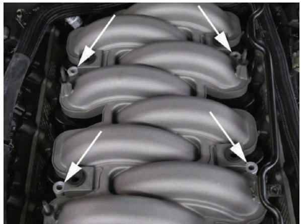
Fig. 9H: Aluminum Fuel Rail Spacers
