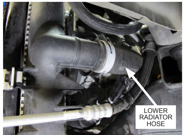
Fig. 2-q: Detach lower radiator hose
