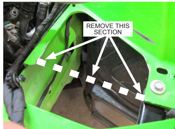
Fig. 7-b: Modify driver side inner wheel well as shown
