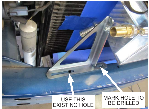
Fig. 7-p: Mark the holes to be drilled on the passenger side of the front bumper support
