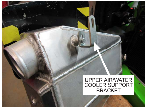
Fig. 7-n: Install upper air/water cooler support bracket
