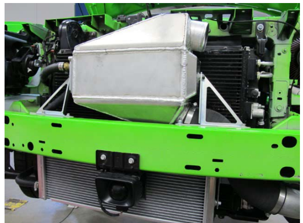
Fig. 7-x: Install air/water cooler
