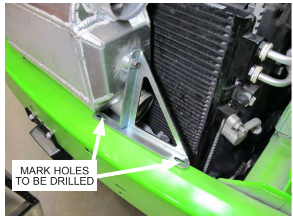
Fig. 7-q: Mark the two holes to be drilled on the driver side of the front bumper support
