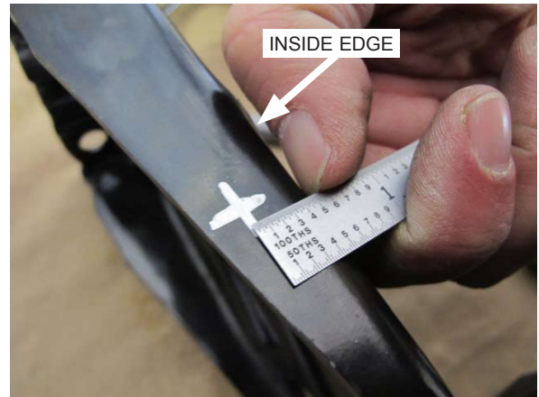
Fig. 4-g: Measure 1/2" from inside edge
