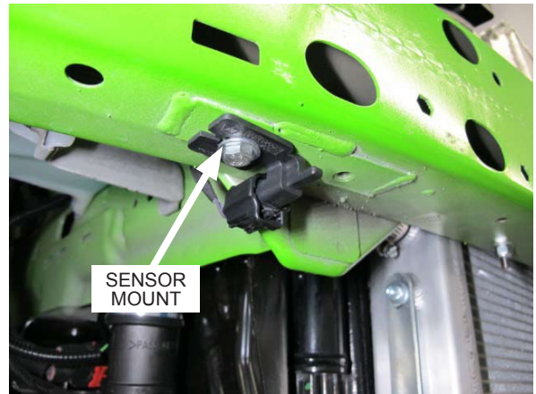
Fig. 7-ah: Reinstall ambient air temperature sensor as shown
