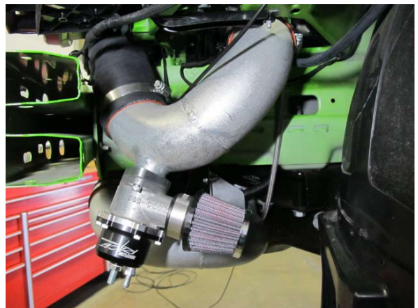
Fig. 7-ag: Loosely install discharge tube 'A' to discharge tube 'B'
