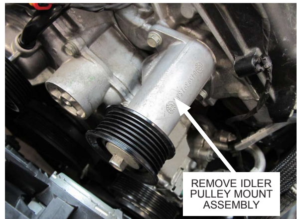
Fig. 2-v: Remove idler pulley mount assembly
