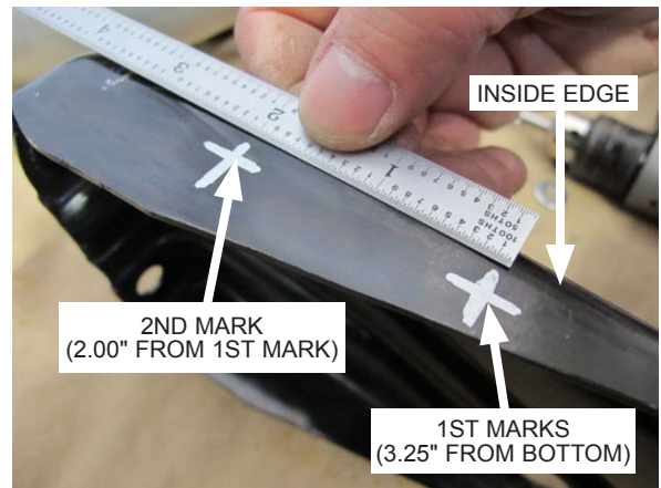
Fig. 4-h: Measure 2.00" up from first marks
