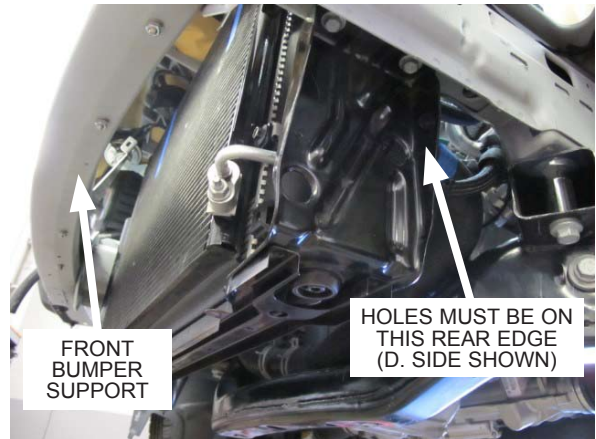
Fig. 4-k: Reinstall lower radiator support
