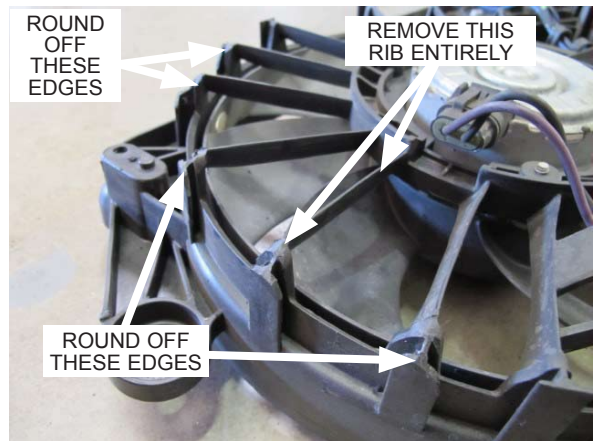
Fig. 4-b: Modify as shown
