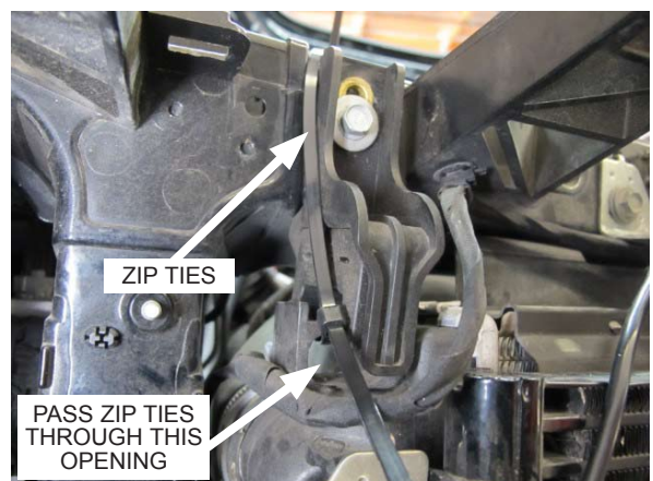
Fig. 2-r: Zip tie radiator to core support
