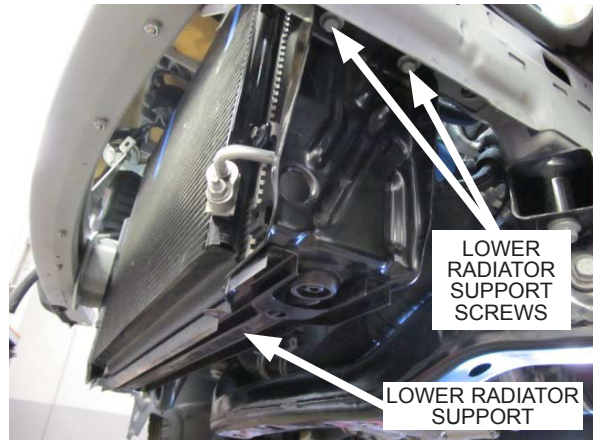
Fig. 2-s: Remove lower radiator support hardware
