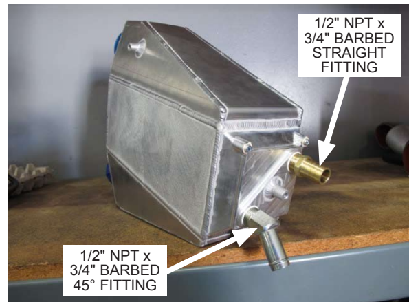
Fig. 7-a: Install fittings to air/water cooler
