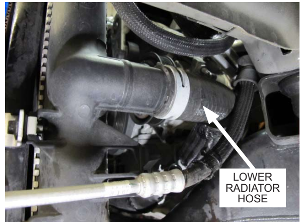
Fig. 4-d: Reattach lower radiator hose
