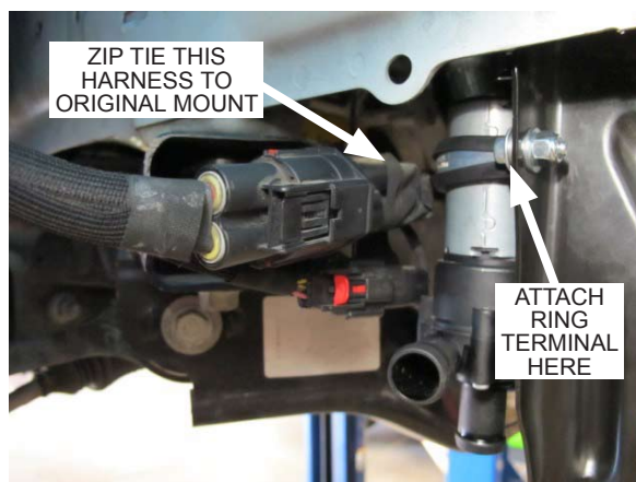
Fig. 9-f: Install the auxiliary water pump
