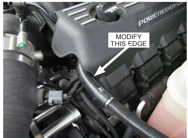
Fig. 10-b: Modify driver side engine cover
