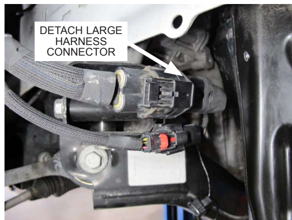
Fig. 9-d: Large harness connector
