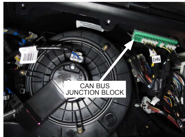
Fig. 14-b: CAN bus junction block
