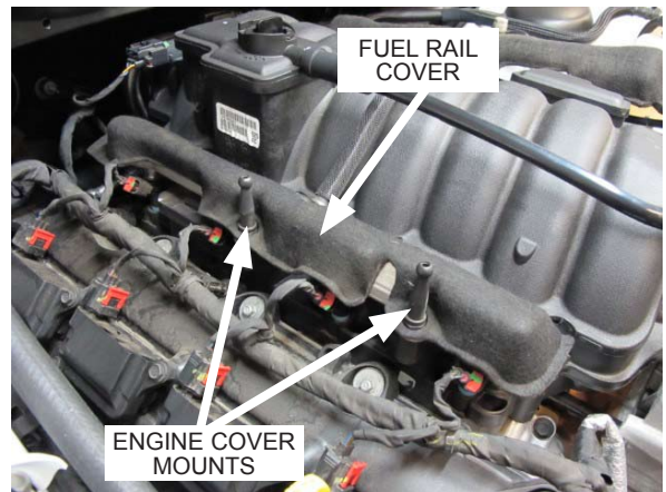
Fig. 11-d: Remove fuel rail covers, engine covers, and engine cover mounts (Passenger side shown)
