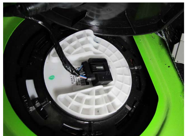
Fig. 12-l: Disconnect fuel pump
