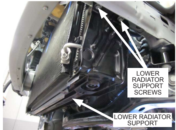
Fig. 2-v: Remove lower radiator support hardware
