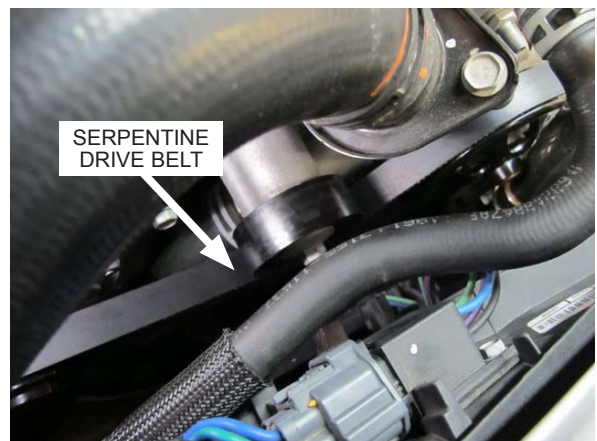
Fig. 6-i: Slide serpentine belt under OEM passenger side smooth idler pulley
