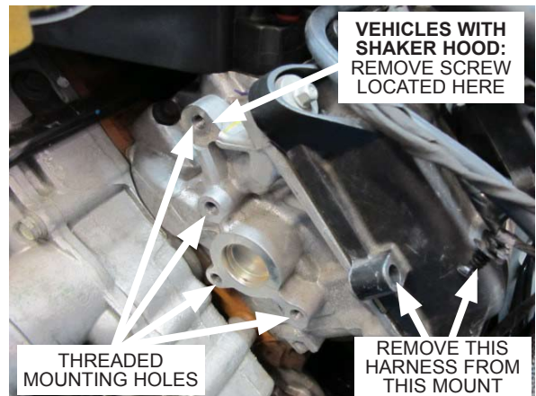
Fig. 6-e: Driver side cylinder head
