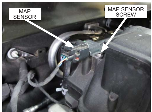
Fig. 11-i: Install 3-Bar MAP sensor
