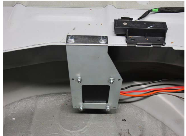
Fig. 12-g: Mount fuel pump booster mounting plate to vehicle
