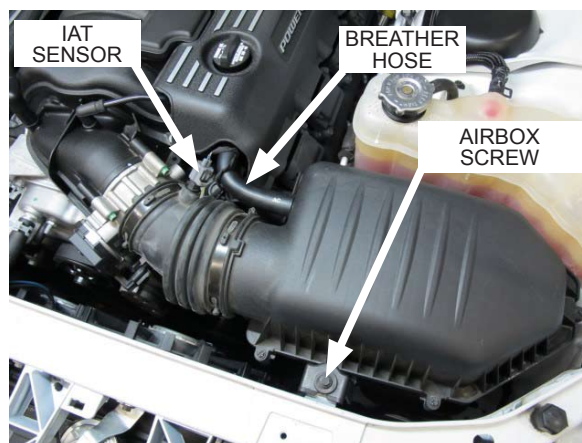
Fig. 2-q: Remove airbox and air inlet duct
