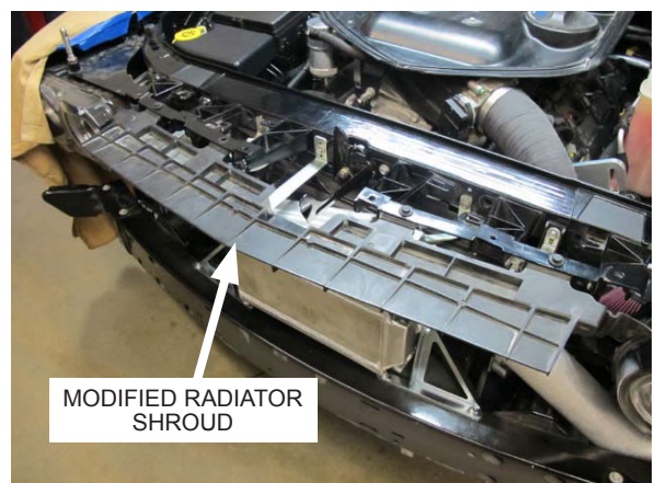
Fig. 10-f: Secure modified radiator shroud and three radiator shroud brackets
