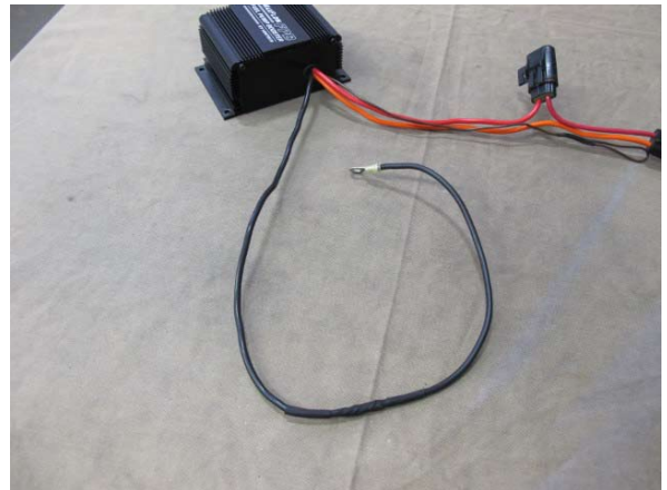
Fig. 12-d: Extend ground wire on fuel pump booster
