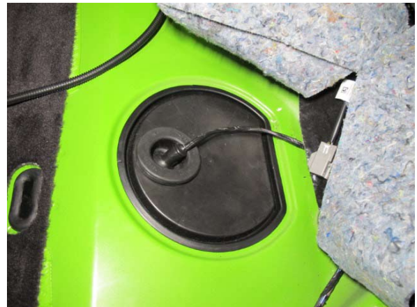
Fig. 12-k: Remove fuel pump access panel
