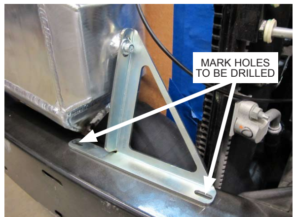
Fig. 7-u: Use driver side air/water cooler support bracket as drill template
