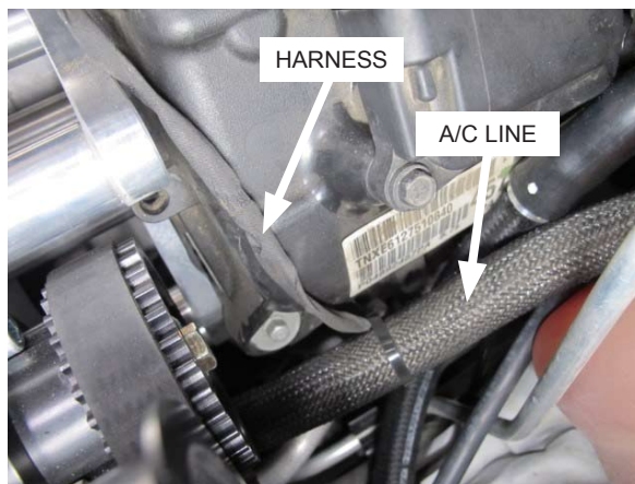
Fig. 6-k: Secure harness to A/C line
