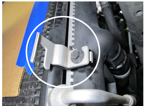
Fig. 7-f: Remove aluminum bracket and screw
