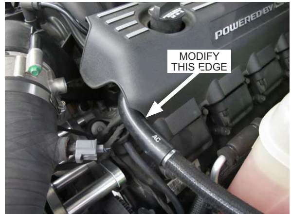
Fig. 13-d: Modify driver side engine cover
