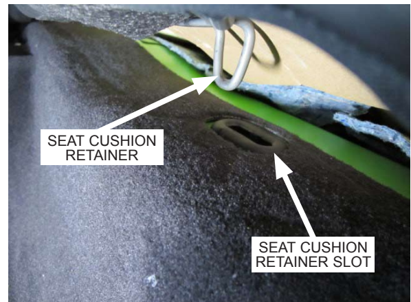
Fig. 12-j: Remove lower rear seat cushion
