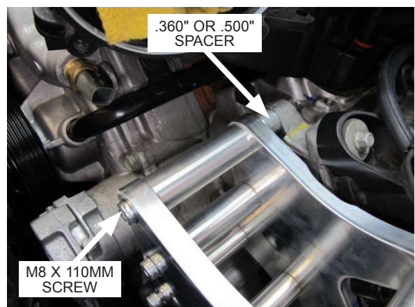
Fig. 6-f: Loosely attach S/C mounting bracket assembly to driver side cylinder head
