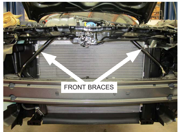
Fig. 4-t: Remove Front Braces
