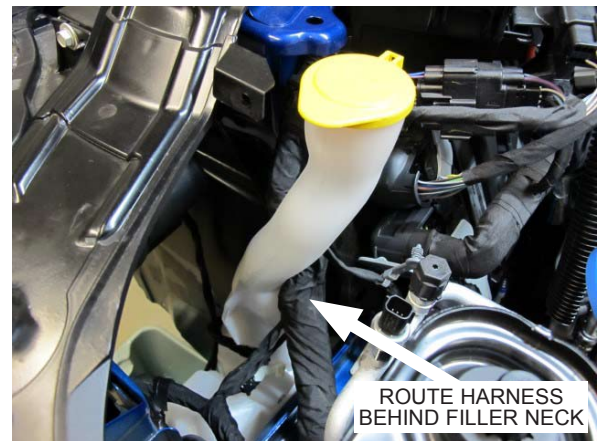
Fig. 4-k: Reinstall Windshield Washer Fluid Reservoir
