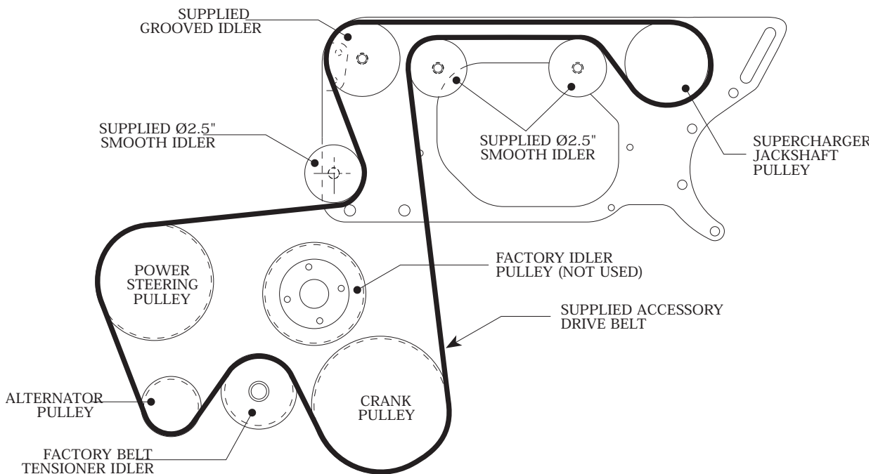
Fig. 6-e / Accessory Drive Belt Routing (300hp Engines)
