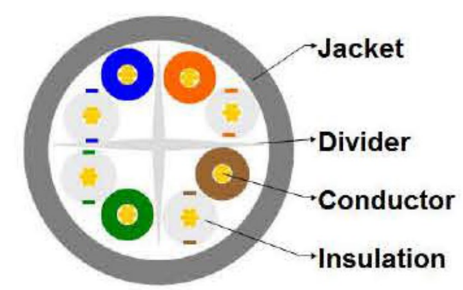
CABLE CROSS-SECTION
