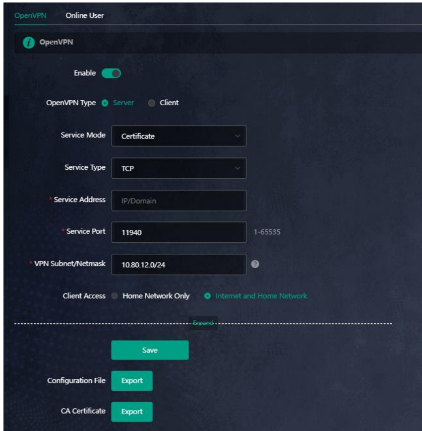
Figure 1-3 Configuring OpenVPN Server
