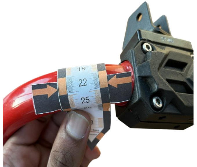
Measuring Tape used on bent pipe surface
