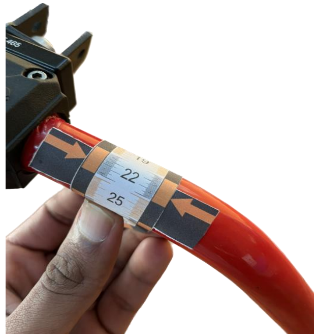
Measuring Tape used on straight pipe surface
