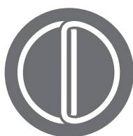
The strongest signal occurs where the Tx and Rx coil windings overlap.
