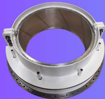
Hydro Bearings
